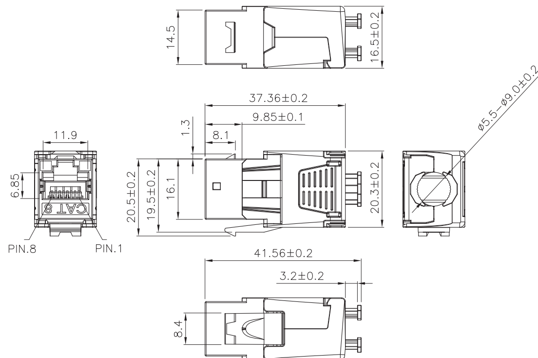
Figure D.2-Panel drawing
